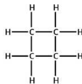
CYCLOBUTANE
