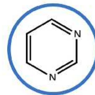
PYRIMIDINE 1,3-diazine C_4H_4N_2
