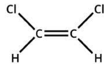
(Z)-1,2-DICHLOROETHENE Z = same side
