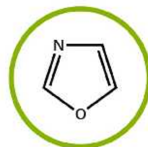
OXAZOLE 1,3-oxazole C_3H_3NO
