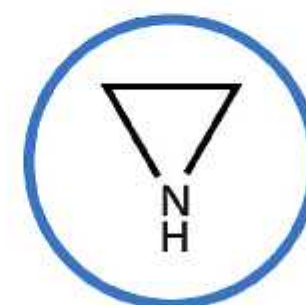
ETHYLENE IMINE Aziridine C_2H_5N
