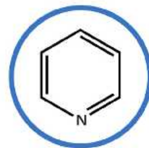
PYRIDINE Azine C_5H_5N
