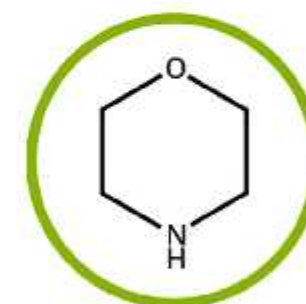
MORPHOLINE Tetrahydro-1,4-oxazine C_4H_9NO
