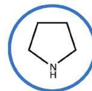
PYRROLIDINE Azolidine C_4H_9N
