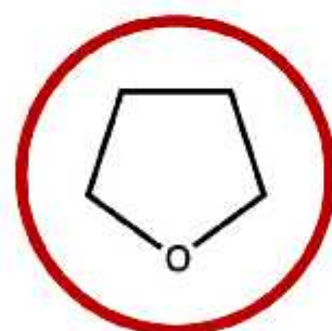
TETRAHYDROFURAN Oxolane C_4H_8O
