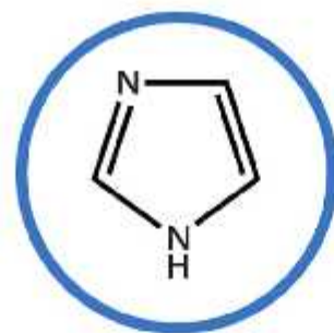
IMIDAZOLE 1,3-diazole C_3H_4N_2
