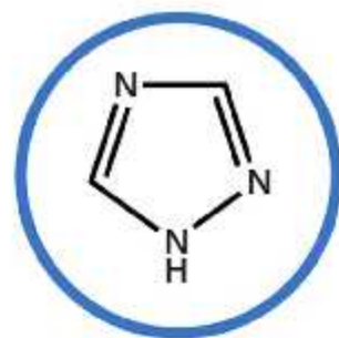
TRIAZOLE 1,2,4-triazole C_2H_3N_3
