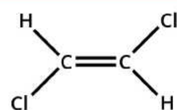
(E)-1,2-DICHLOROETHENE E = opposite side
