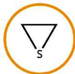
ETHYLENE SULFIDE Thiirane C_2H_4S
