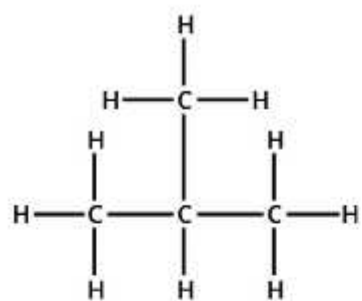
2-METHYL PROPANE
