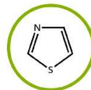
THIAZOLE 1,3-thiazole C_3H_3NS
