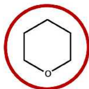
TETRAHYDROPYRAN Oxane C_5H_{10}O
