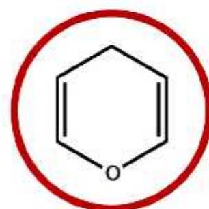
4H-PYRAN 4H-Oxine C_5H_6O
